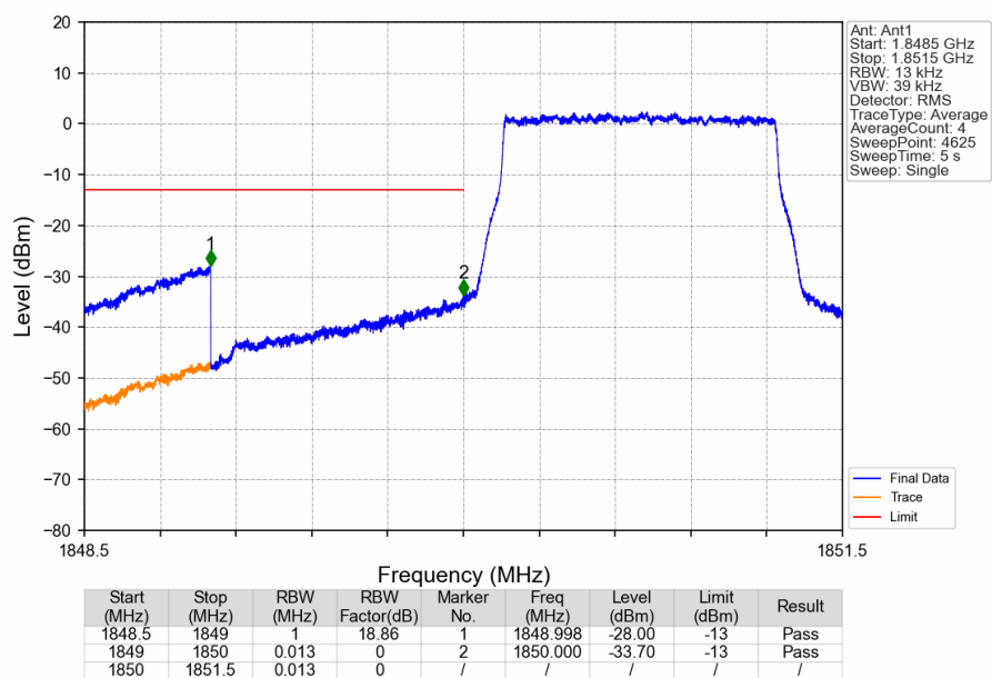
Band2_1.4MHz_16QAM_LCH_1850.7MHz_RB_6_0_NTNV
