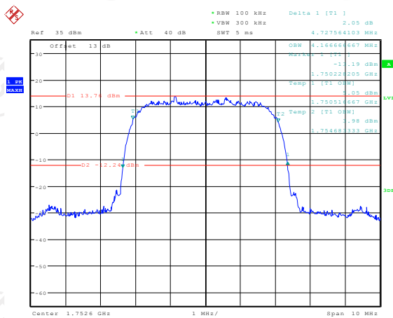
26dB&99% Occupied Bandwidth Plot on Channel 1513
