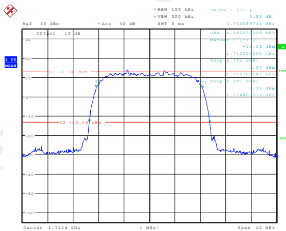
26dB&99% Occupied Bandwidth Plot on Channel 1312
