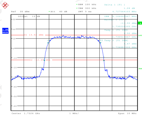
26dB&99% Occupied Bandwidth Plot on Channel 1413
