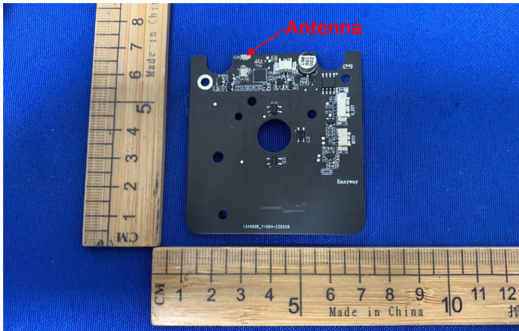
Figure 7. Internal view
