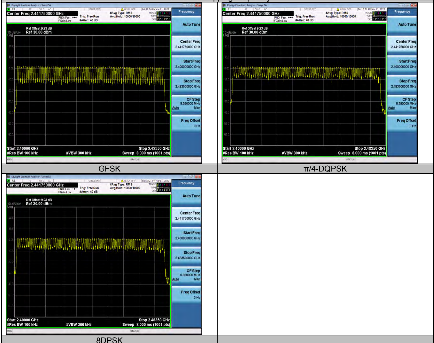
Number of hopping frequency
