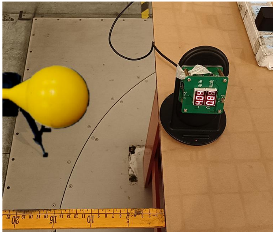
Test Position E - Exposure photo from side edge surface-Right(TM1) - 15 cm
