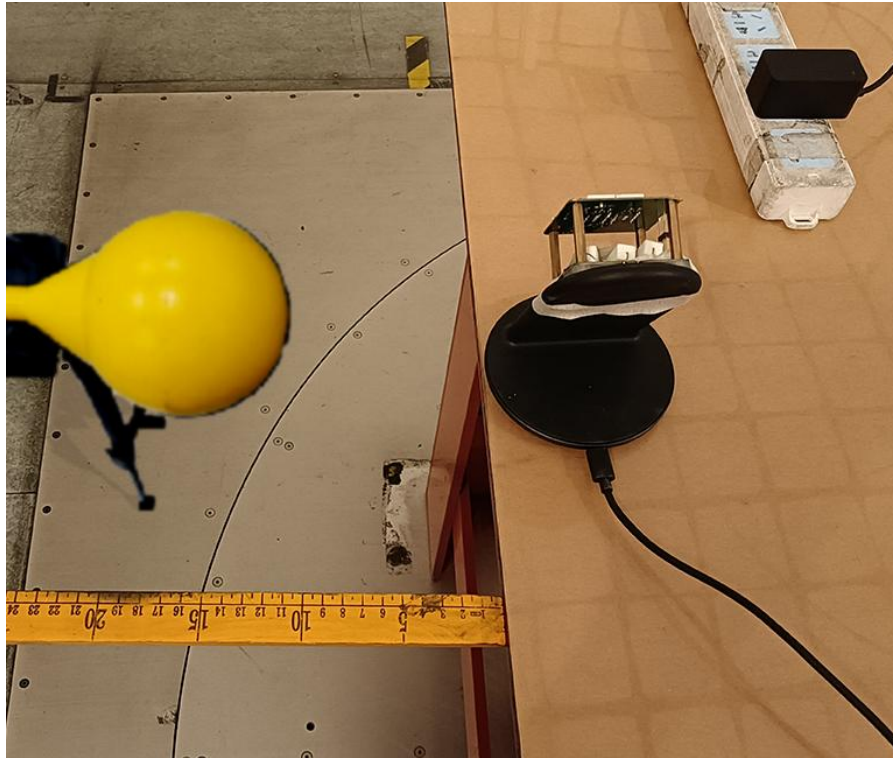
Test Position C - Exposure photo from side edge surface-Left(TM1) - 15 cm
