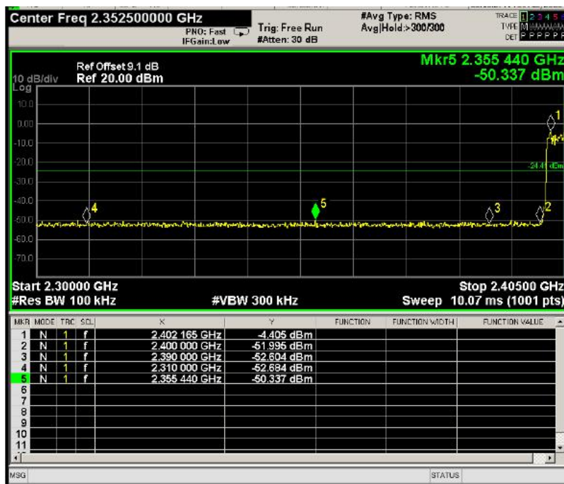
For Hopping Mode (EDR)
