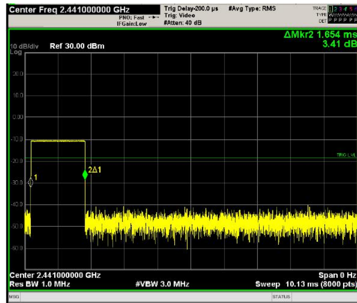
Test Mode: EDR---3DH3
