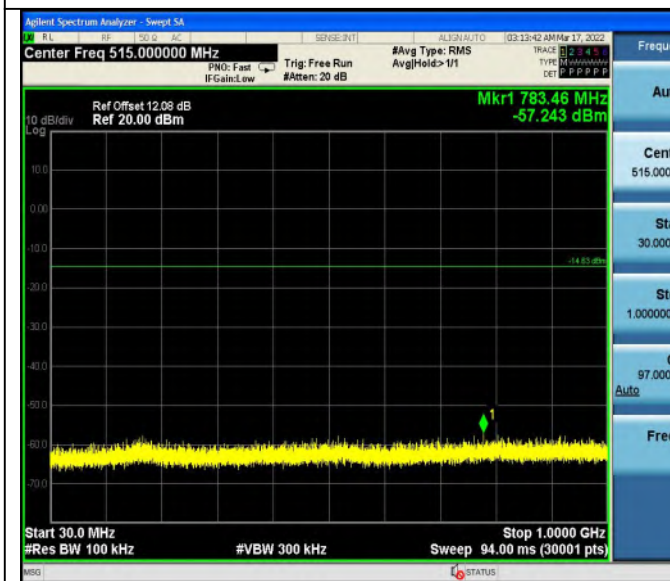
DH5_Ant1_2402_30~1000
