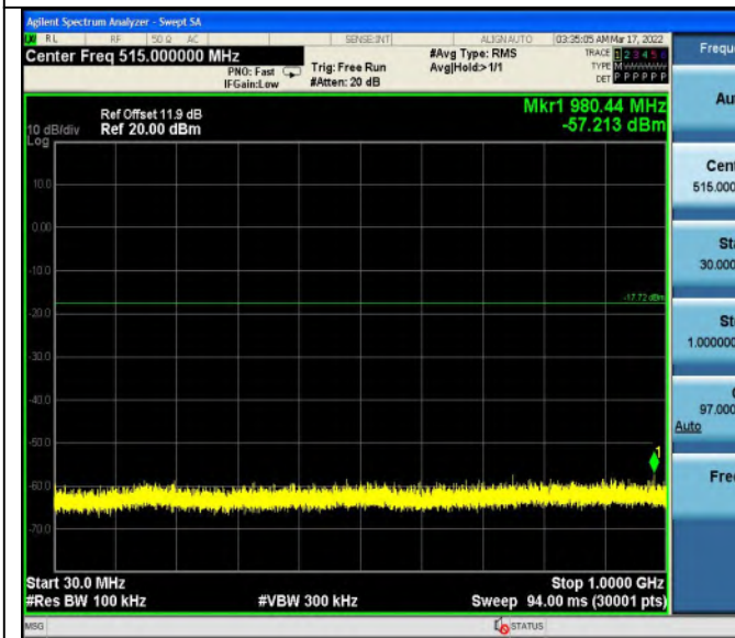
2DH5_Ant1_2480_30~1000
