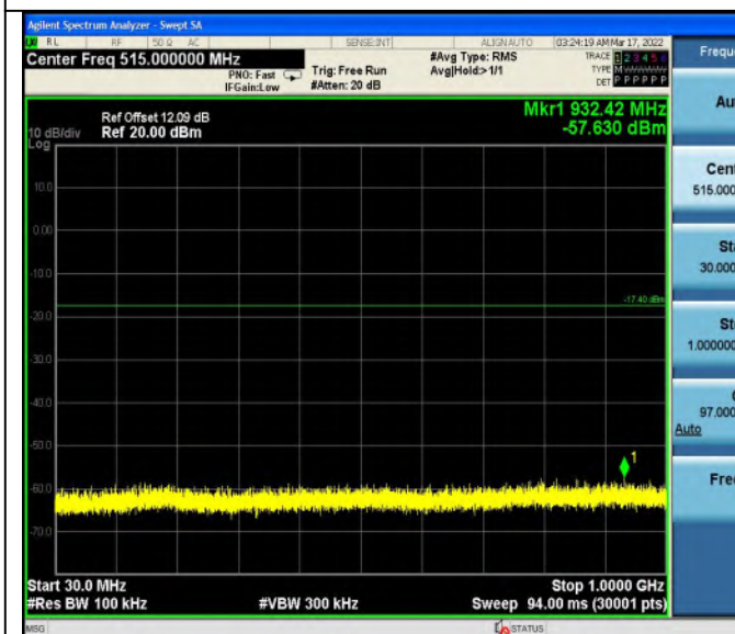
2DH5_Ant1_2402_30~1000
