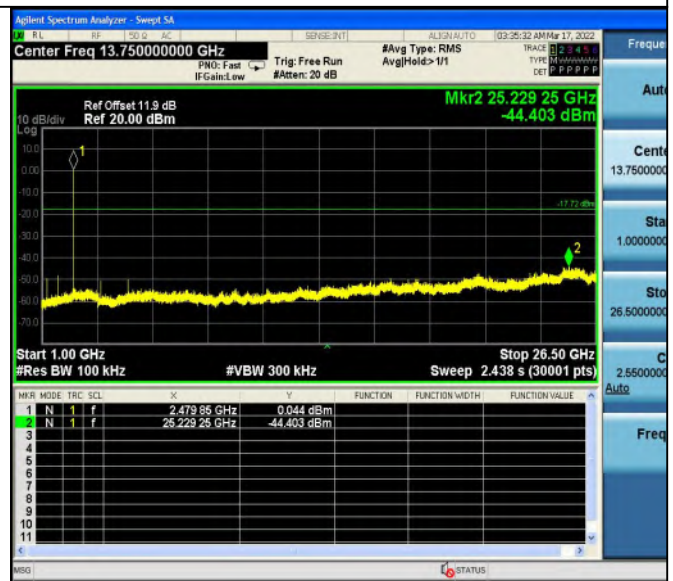
2DH5_Ant1_2480_1000~26500
