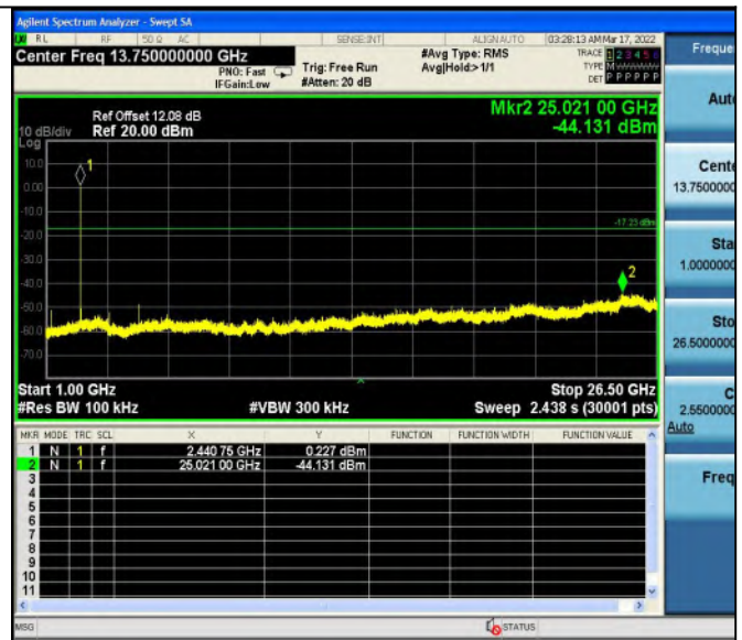
2DH5_Ant1_2441_1000~26500
