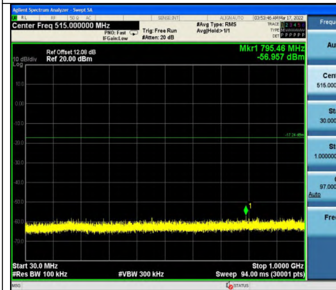
3DH5_Ant1_2441_30~1000
