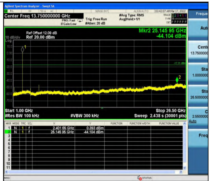
3DH5_Ant1_2402_1000~26500
