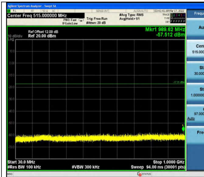
3DH5_Ant1_2402_30~1000
