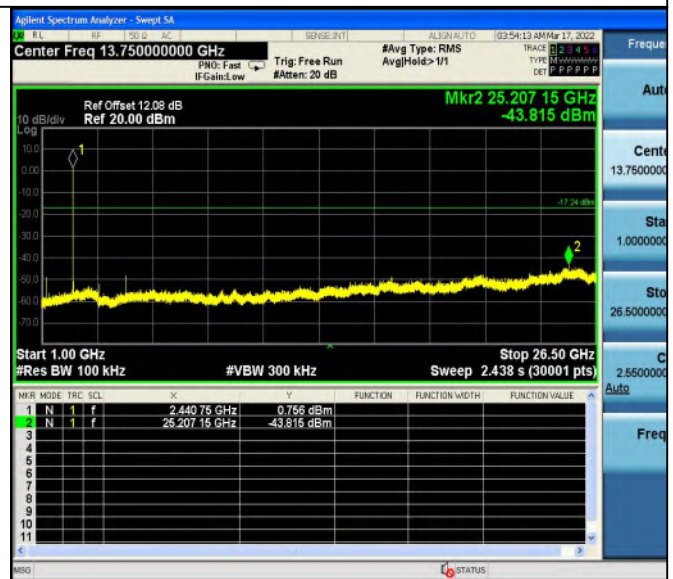
3DH5_Ant1_2441_1000~26500
