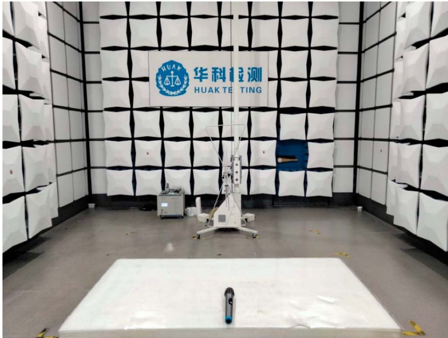
PWMA1099A Radiated Emissions
