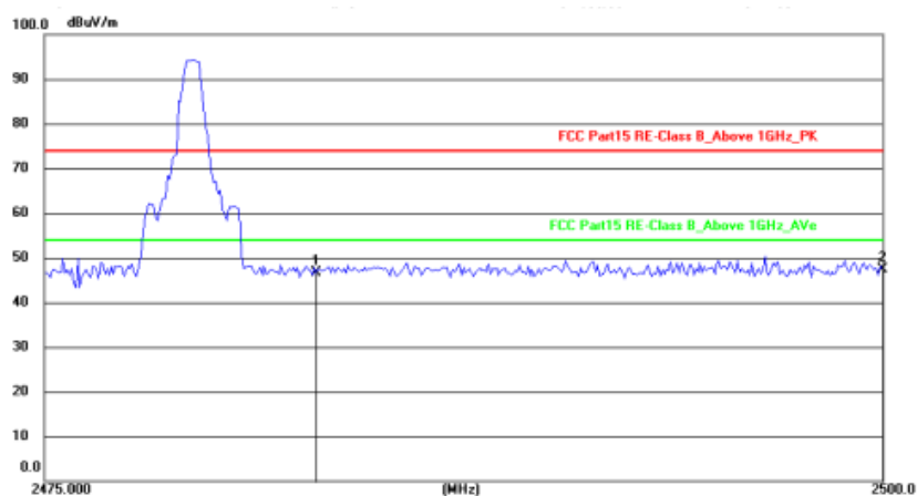
2480MHz Vertical
