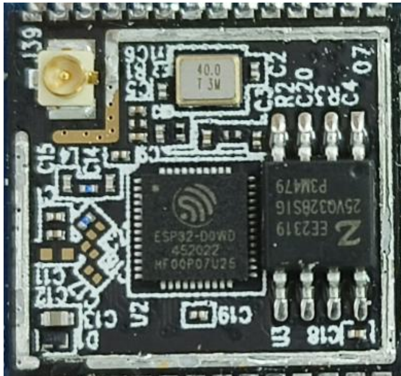
Internal photograph of EUT
