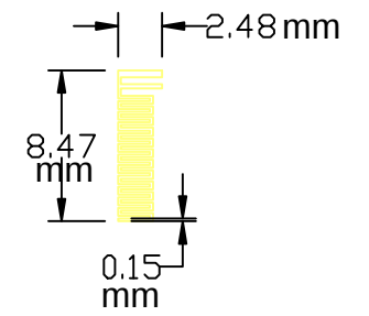
MP200 Bluetooth Antenna
