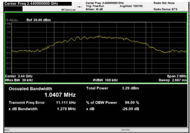
Bluetooth LE Carrier frequency (MHz): 2440
