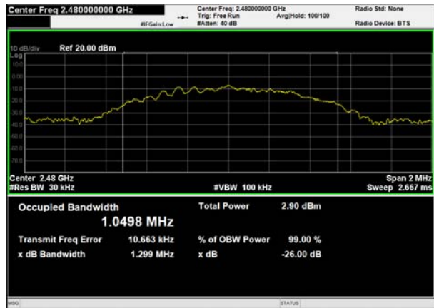
Bluetooth LE Carrier frequency (MHz): 2480
