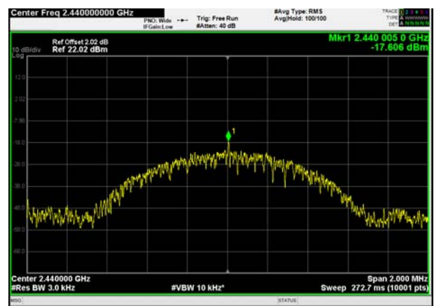
Bluetooth LE, Channel No.: 19
