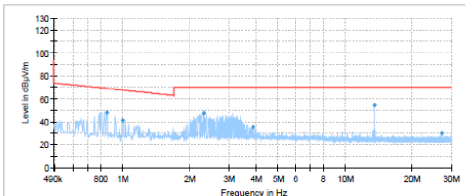
Radiates Emission from 490kHz to 30MHz
