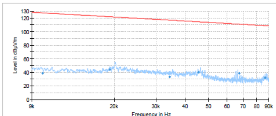
Radiates Emission from 9kHz to 90kHz
