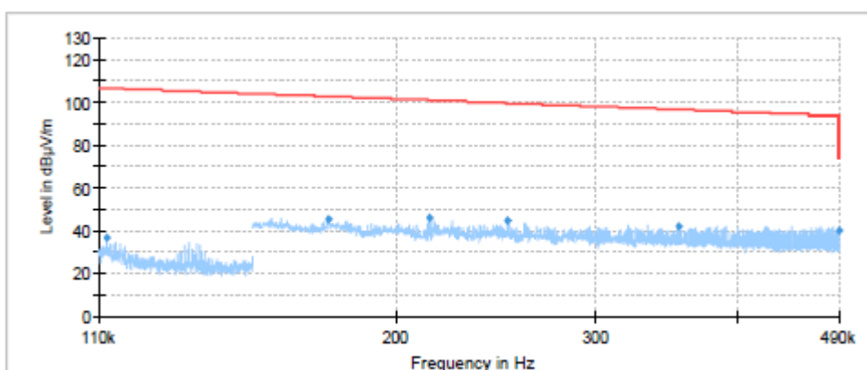
Radiates Emission from 110kHz to 490kHz
