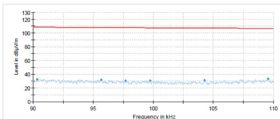
Radiates Emission from 90kHz to 110kHz
