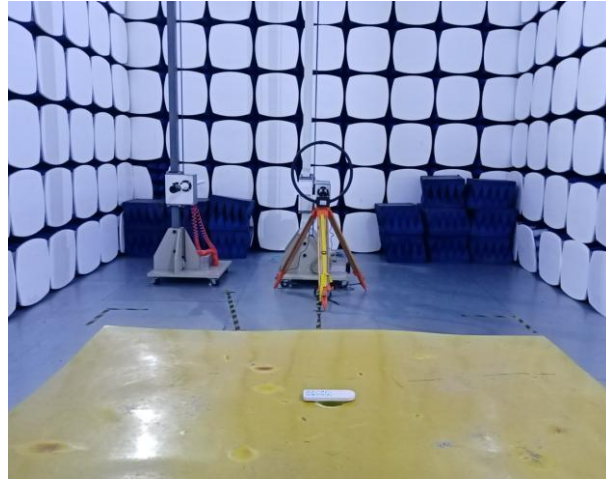
Radiated emission Below 30MHz
