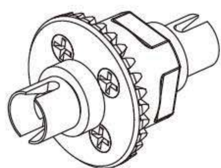
金属差速器总成(无刷) Components differential (Brushless)
