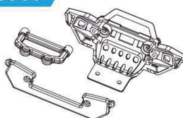
18108前防撞组件 18108 Front bumper assembly
