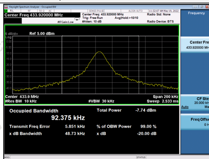
Test plot as follows: ASK Modulation
