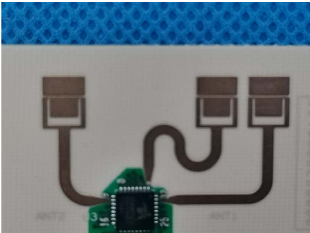
24GHz Antenna
