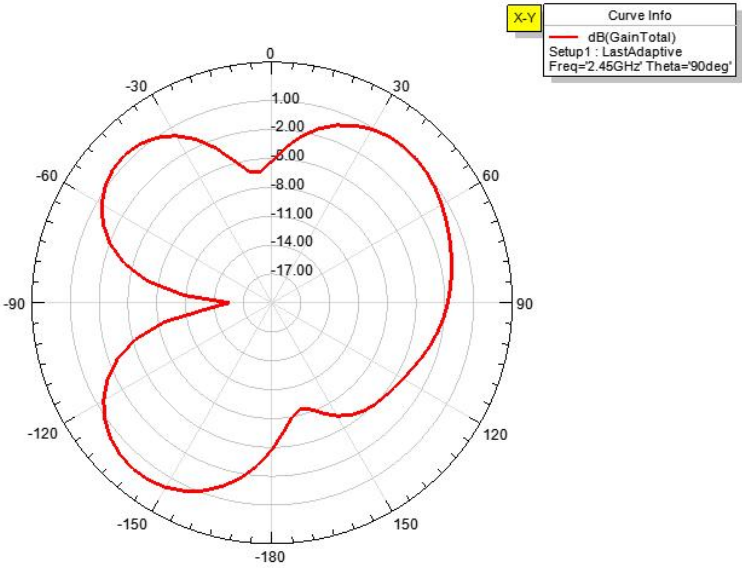
Radiation Pattern 2
