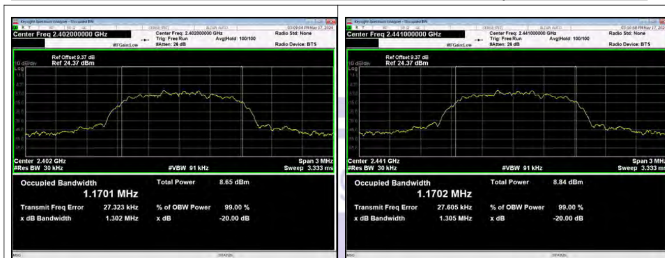
8DPSK_3-DH1_Channel 0
