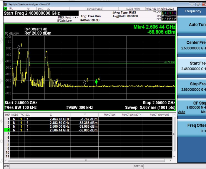
2.4G_Ant1_High_Hop_2479
