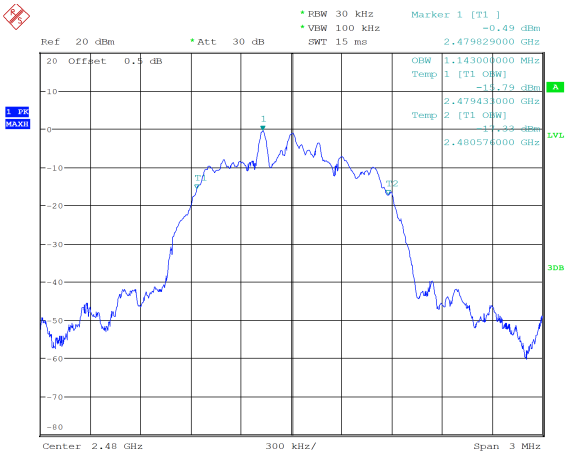
8DPSK_High 1.143 MHz
