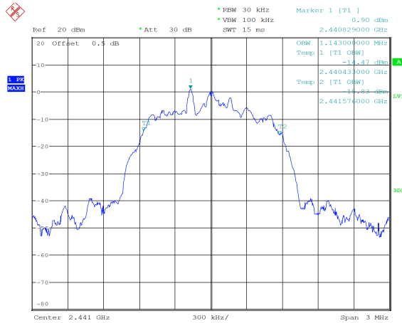
8DPSK_Middle 1.143 MHz
