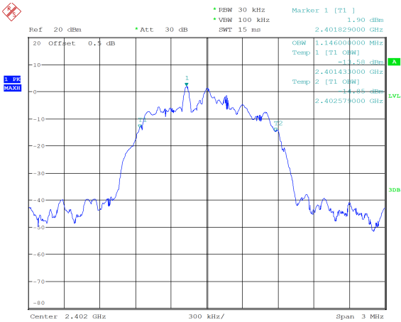
8DPSK_Low 1.146 MHz
