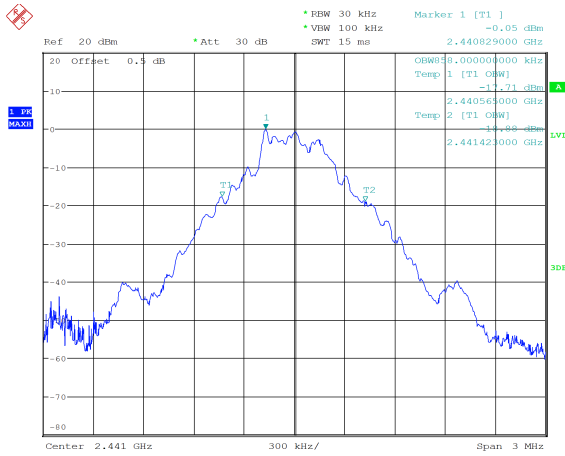
GFSK_Middle 0.858 MHz
