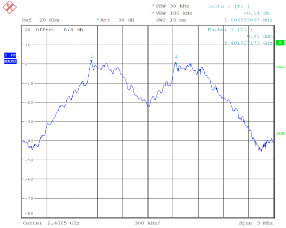
GFSK_Low 1.007 MHz
