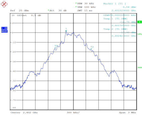
GFSK_Low 0.858 MHz
