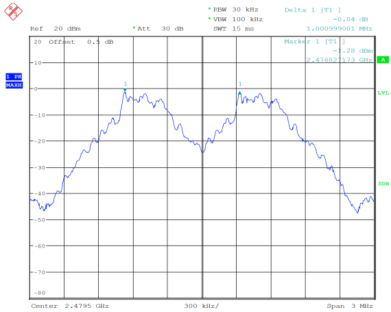
GFSK_High 1.001 MHz
