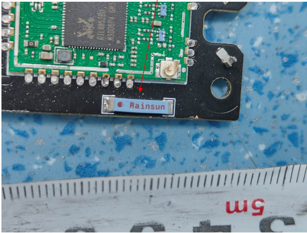
Bluetooth Antenna
