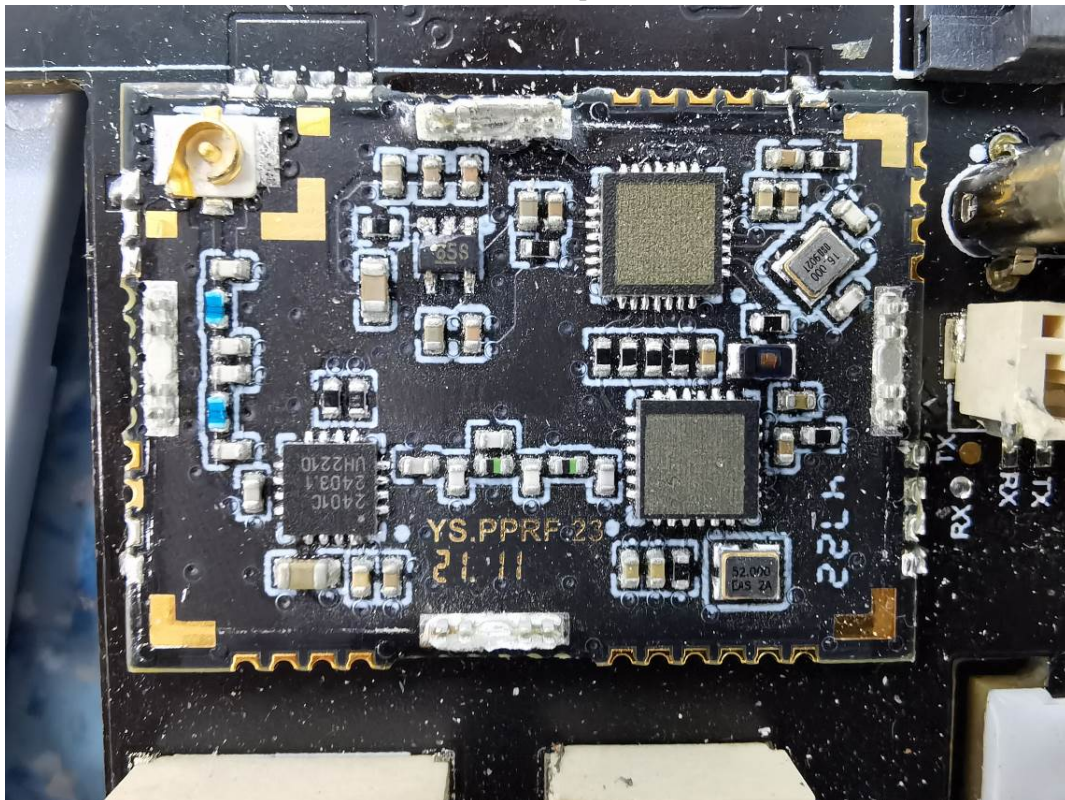
SRD chip
