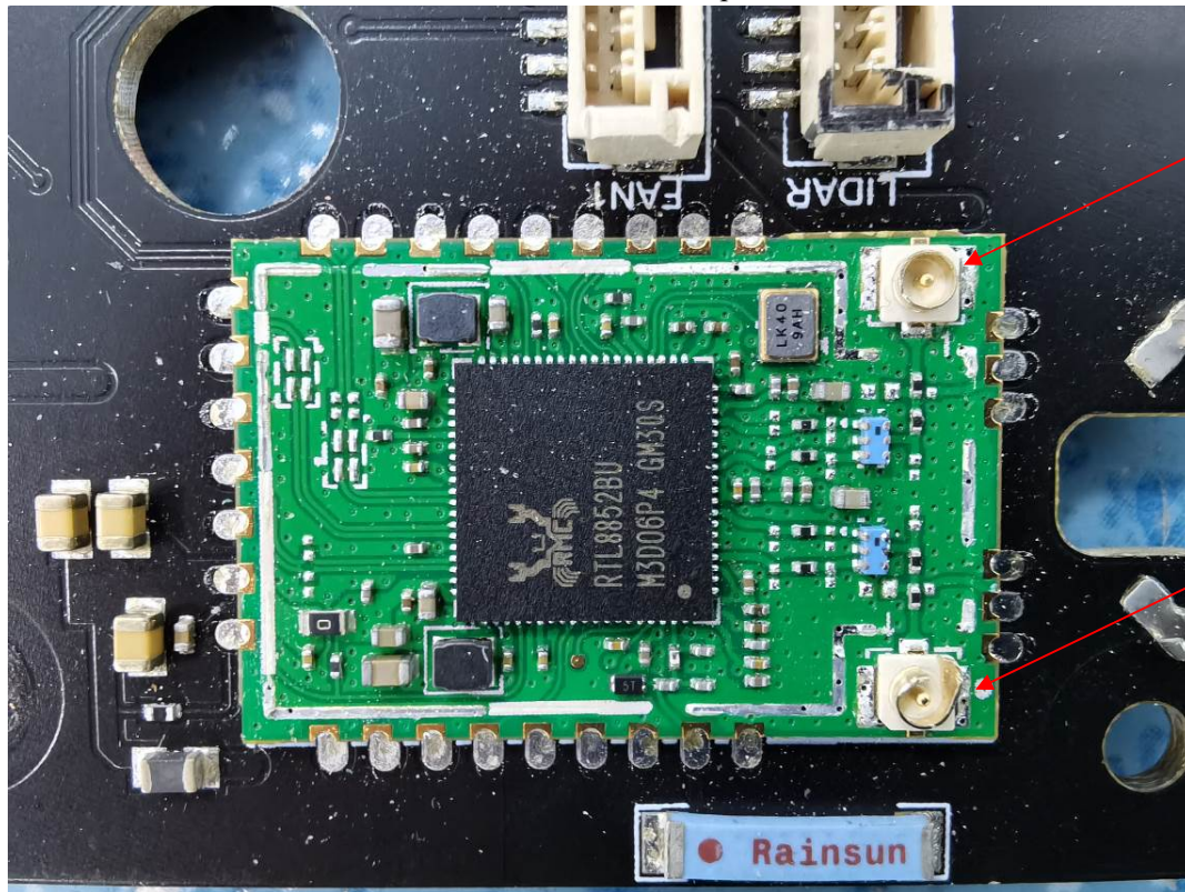
WiFi/Bluetooth Chip
