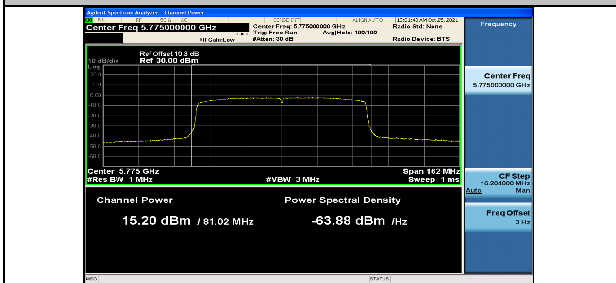
Maximum Conduct Output Power_11AC80_5775_Ant2
