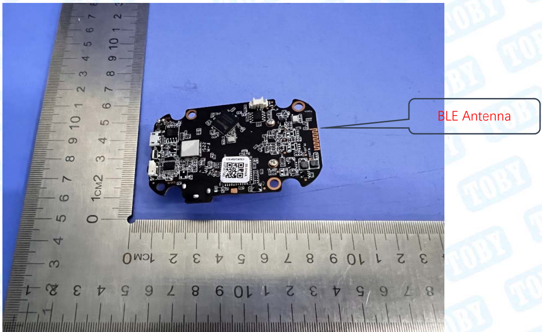
Photo 11 Appearance of PCB
