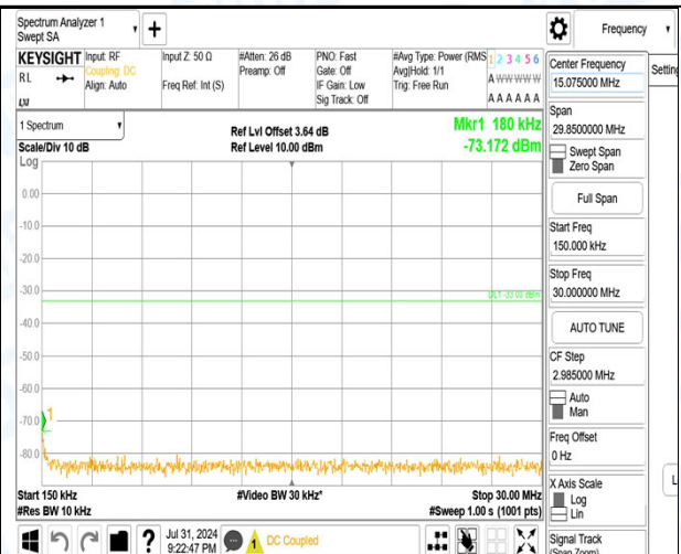
Band4_5MHz_QPSK_19975_1RB#0_1000~3000_1000~3000
