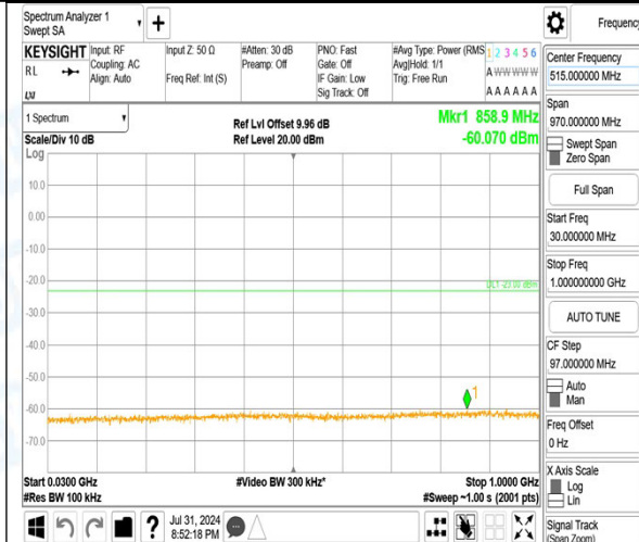
Band4_3MHz_QPSK_19965_15RB#0_3000~20000_3000~20000
