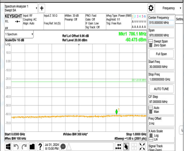
Band4_1.4MHz_16QAM_19957_6RB#0_3000~20000_3000~20000 0
