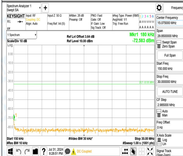
Band4_1.4MHz_16QAM_20393_6RB#0_0.15~30_0.15~30
