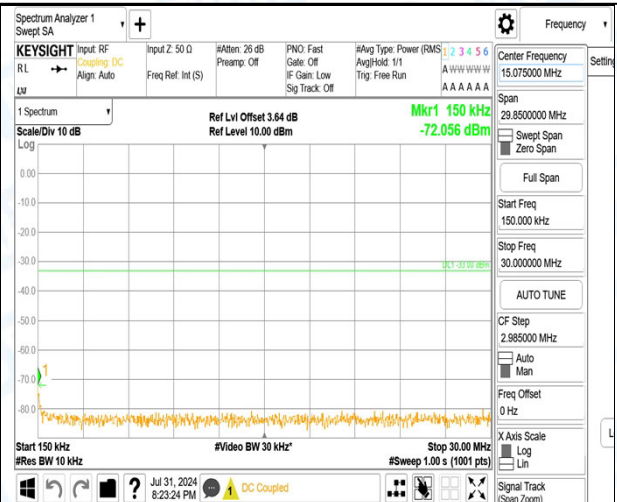
Band4_1.4MHz_QPSK_20393_1RB#0_1000~3000_1000~3000
