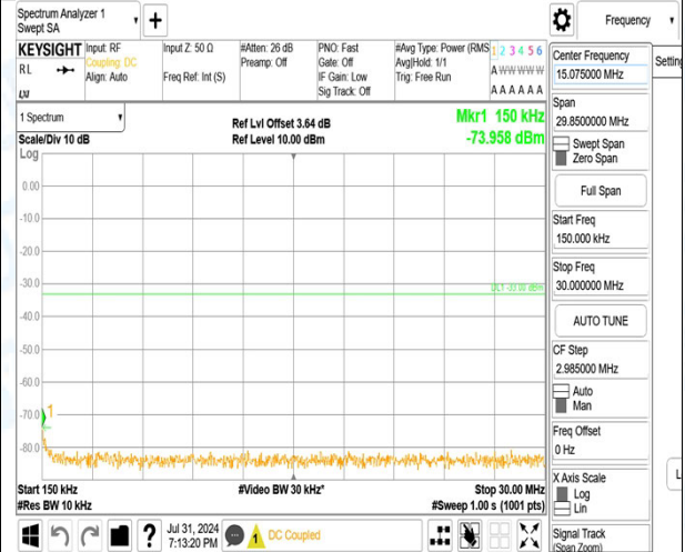
Band2_15MHz_16QAM_18900_1RB#0_1000~3000_1000~3000
