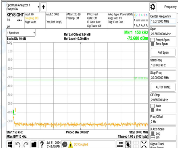
Band2_20MHz_QPSK_18900_1RB#0_1000~3000_1000~3000
