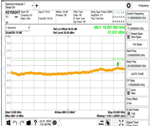
Band2_20MHz_QPSK_18900_1RB#0_0.15~30_0.15~30
