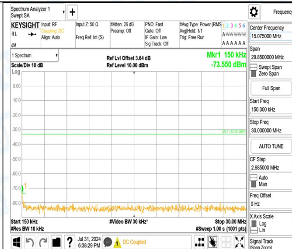
Band2_10MHz_16QAM_19150_1RB#0_1000~3000_1000~3000
