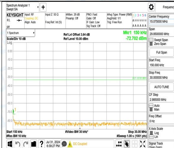
Band2_10MHz_QPSK_19150_1RB#49_1000~3000_1000~3000
