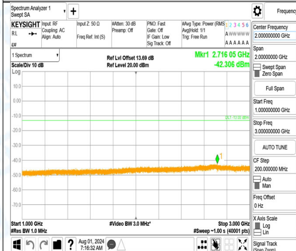
Band13_5MHz_QPSK_23205_25RB#0_0.009~0.15_0.009~0.15
