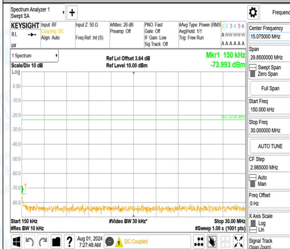
Band13_5MHz_QPSK_23230_25RB#0_0.15~30_0.15~30
