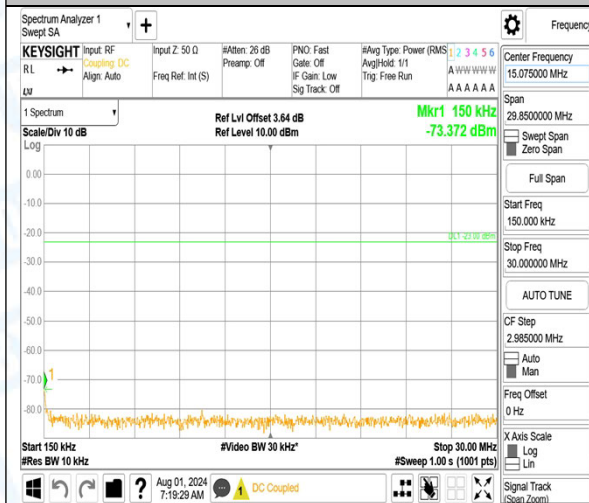
Band13_5MHz_16QAM_23205_25RB#0_0.15~30_0.15~30
