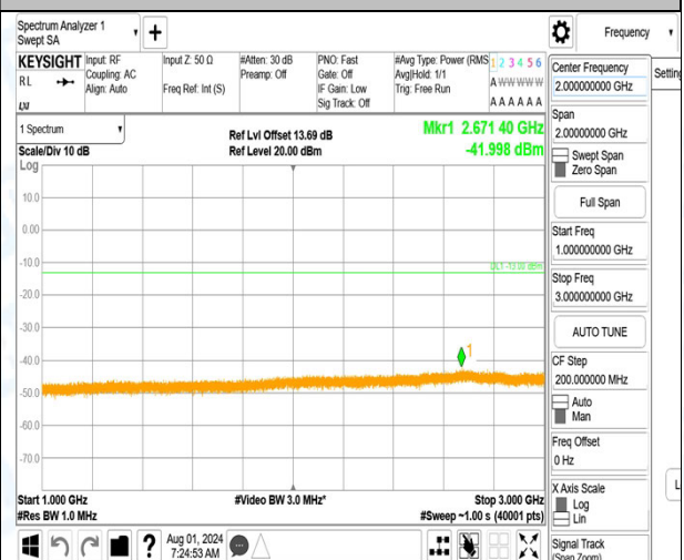
Band13_5MHz_16QAM_23230_1RB#0_1000~3000_1000~3000
