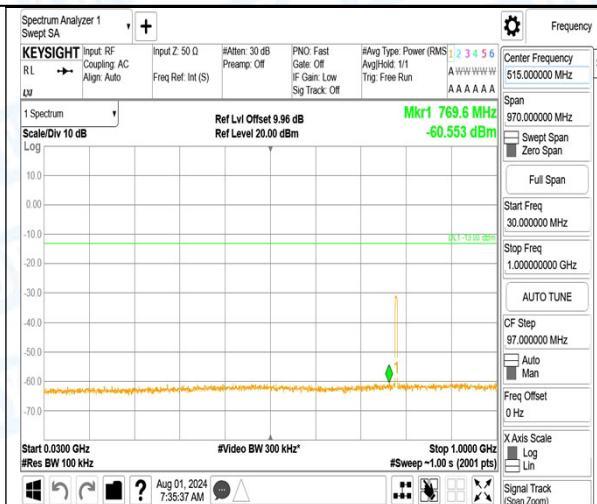
Band13_5MHz_QPSK_23255_25RB#0_3000~10000_3000~1000
