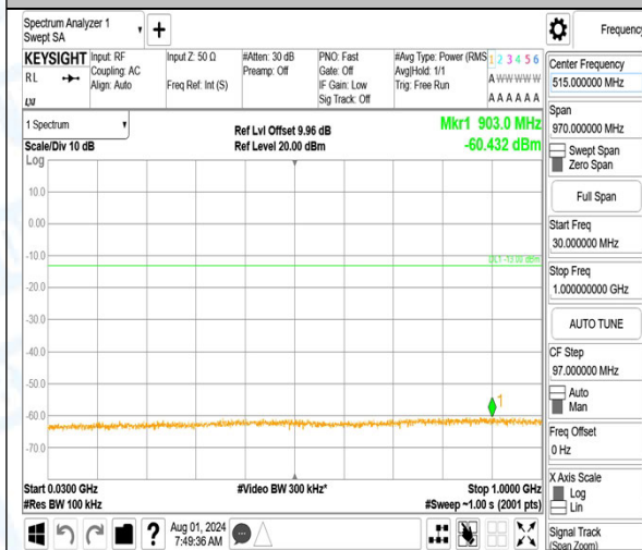
Band13_10MHz_QPSK_23230_1RB#0_3000~10000_3000~1000
