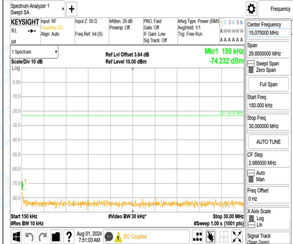
Band13_10MHz_16QAM_23230_1RB#0_1000~3000_1000~3000
