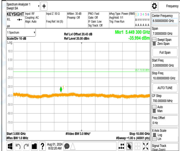
Band13_10MHz_16QAM_23230_1RB#0_0.15~30_0.15~30
