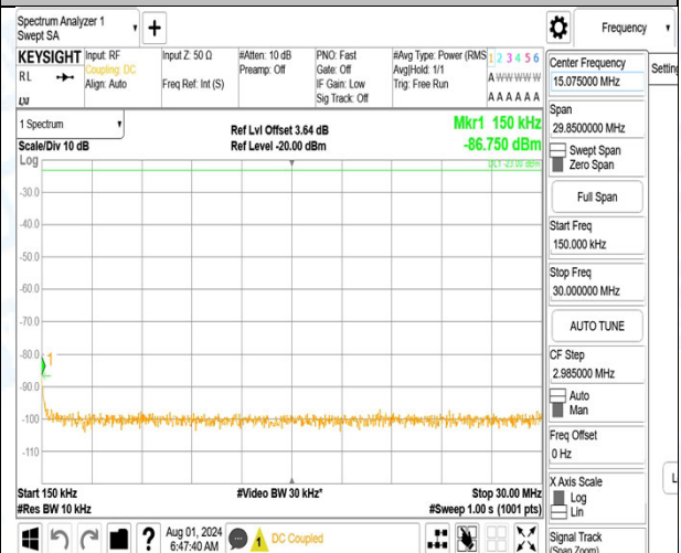
Band12_10MHz_16QAM_23130_1RB#49_1000~3000_1000~3000 0
