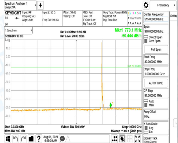
Band12_10MHz_QPSK_23095_1RB#0_3000~10000_3000~10000
