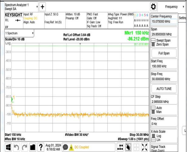
Band12_10MHz_16QAM_23060_1RB#49_1000~3000_1000~300
