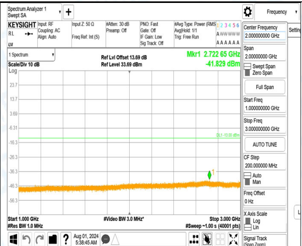
Band12_5MHz_16QAM_23155_1RB#0_0.009~0.15_0.009~0.15
