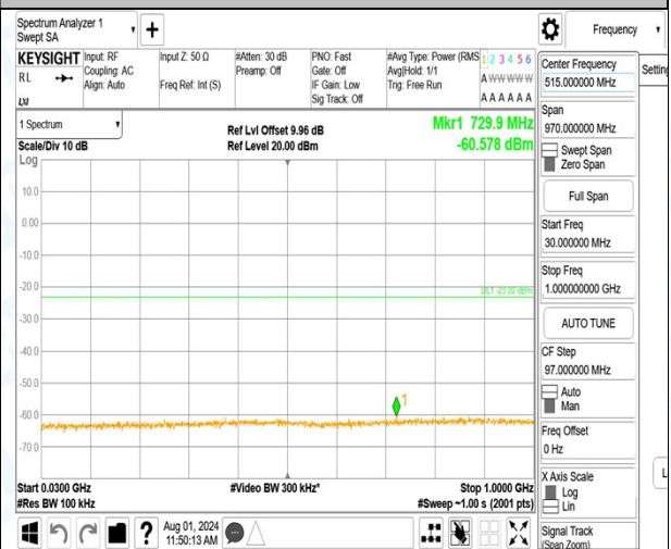
Band66_15MHz_QPSK_132597_75RB#0_3000~20000_3000~20
