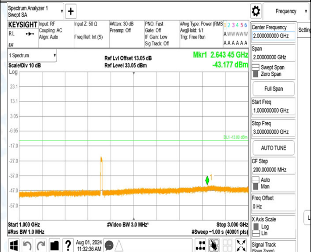
Band66_15MHz_16QAM_132047_1RB#74_0.009~0.15_0.009~0.15
