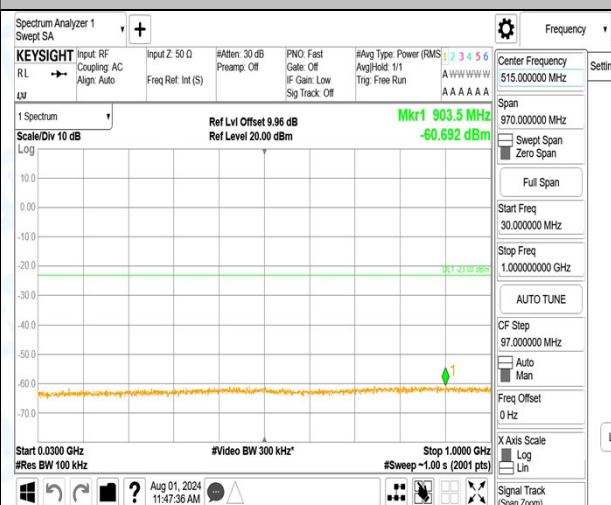
Band66_15MHz_QPSK_132047_75RB#0_3000~20000_3000~20
