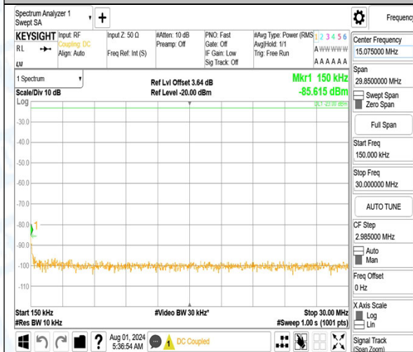
Band12_5MHz_QPSK_23095_25RB#0_0.15~30_0.15~30
