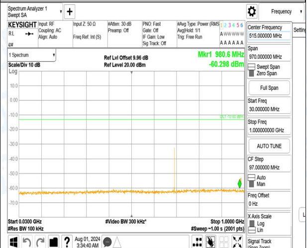
Band12_1.4MHz_16QAM_23017_1RB#0_3000~10000_3000~1000
