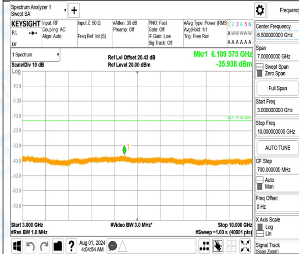
Band12_1.4MHz_16QAM_23173_1RB#0_0.15~30_0.15~30
