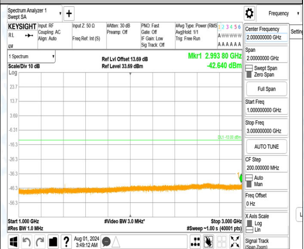
Band12_1.4MHz_16QAM_23095_1RB#0_1000~3000_1000~3000
