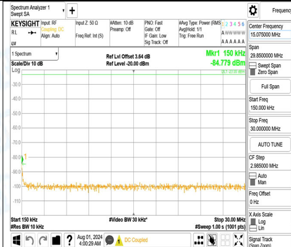
Band12_1.4MHz_16QAM_23095_1RB#5_1000~3000_1000~3000
