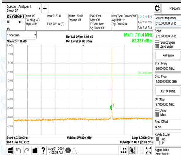
Band12_1.4MHz_QPSK_23173_1RB#0_3000~10000_3000~1000
