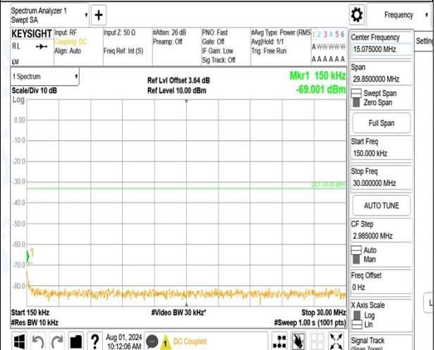
Band66_5MHz_QPSK_132647_25RB#0_1000~3000_1000~3000
