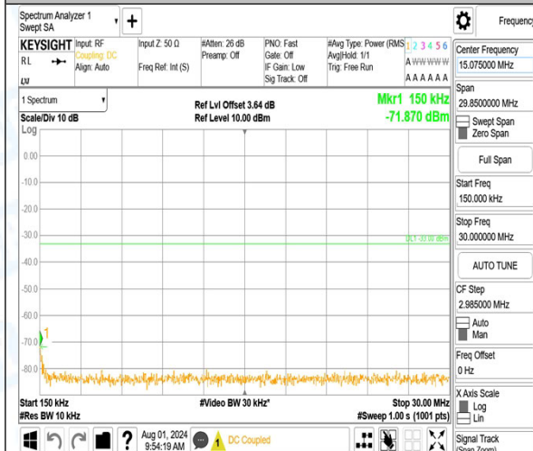
Band66_5MHz_16QAM_131997_1RB#0_0.15~30_0.15~30
