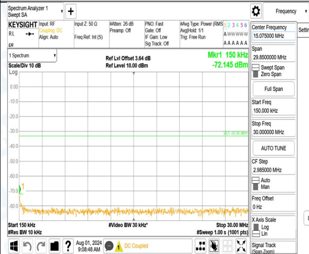
Band66_3MHz_16QAM_131987_1RB#14_1000~3000_1000~300
