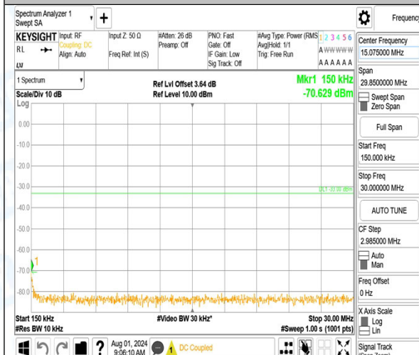
Band66_3MHz_16QAM_131987_1RB#0_0.15~30_0.15~30
