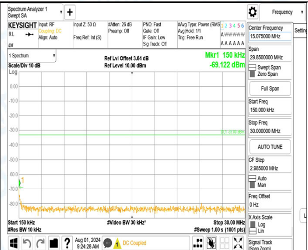
Band66_3MHz_QPSK_132657_1RB#0_1000~3000_1000~3000
