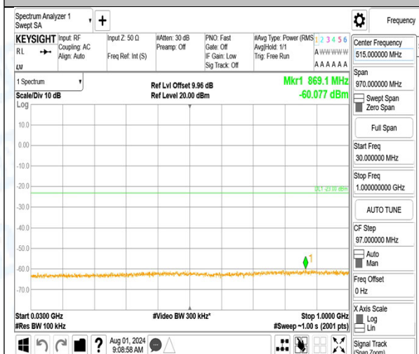
Band66_3MHz_16QAM_131987_1RB#14_3000~20000_3000~20
