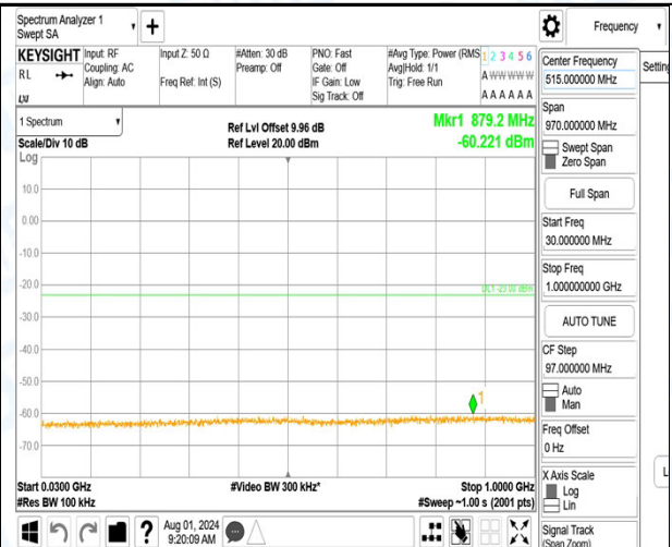
Band66_3MHz_16QAM_132322_1RB#14_3000~20000_3000~20
