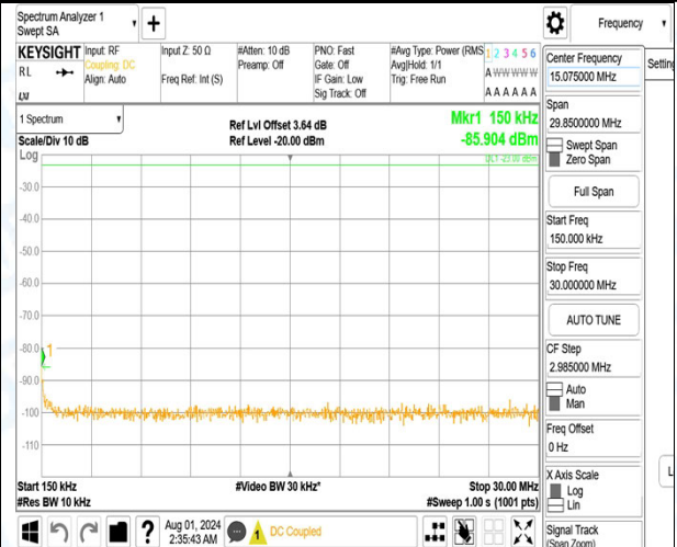
Band5_10MHz_QPSK_20450_1RB#0_1000~3000_1000~3000
