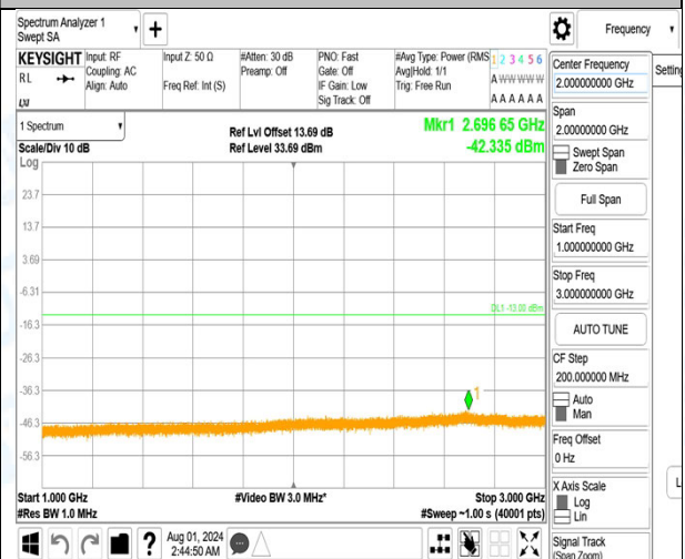
Band5_10MHz_16QAM_20450_1RB#49_1000~3000_1000~3000
