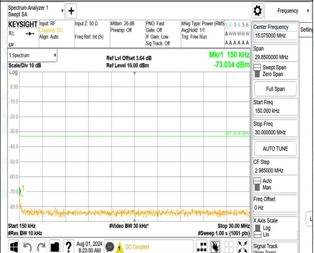
Band66_1.4MHz_QPSK_131979_6RB#0_1000~3000_1000~3000
