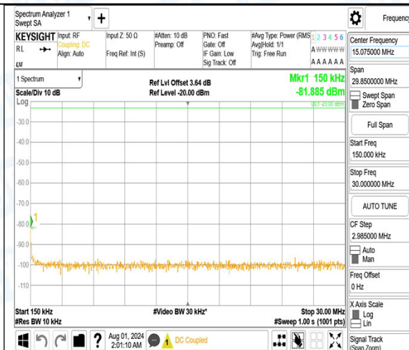
Band5_5MHz_QPSK_20625_1RB#24_1000~3000_1000~3000
