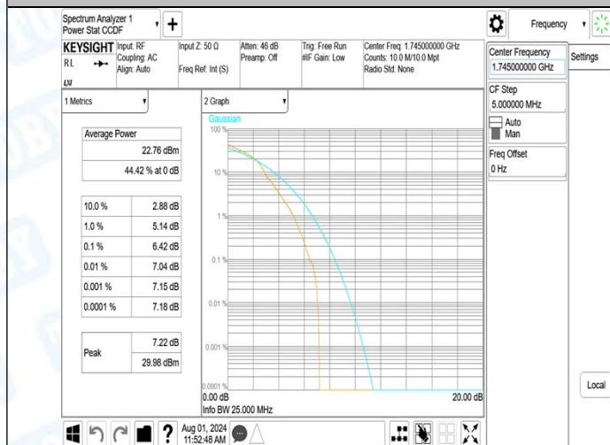
Band66-15MHz-16QAM-132597-1RB#0-PASS
