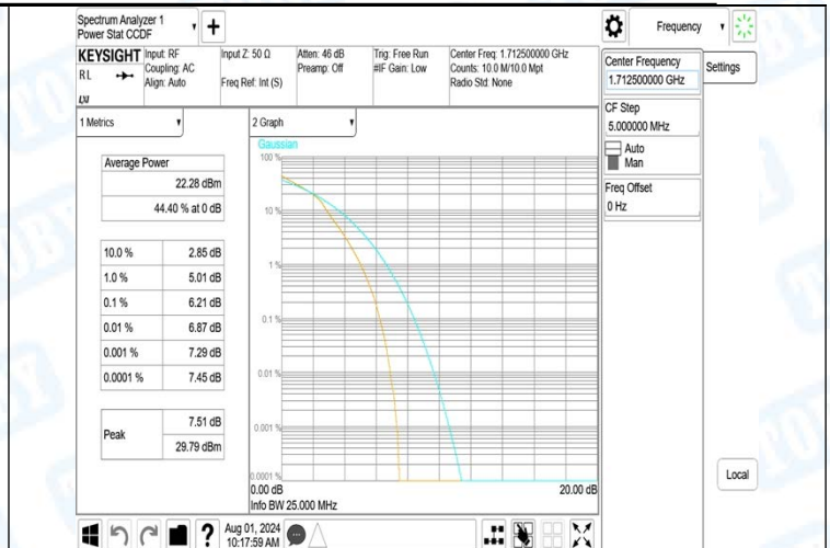
Band66-5MHz-16QAM-132322-25RB#0-PASS
