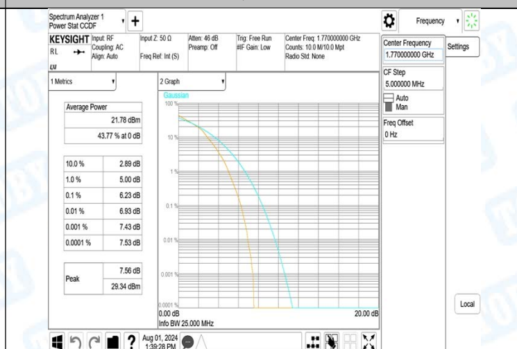
Band66-20MHz-16QAM-132572-27RB#0-PASS
