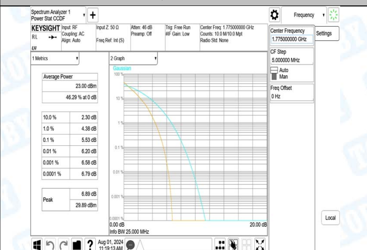
Band66-10MHz-16QAM-132022-27RB#0-PASS
