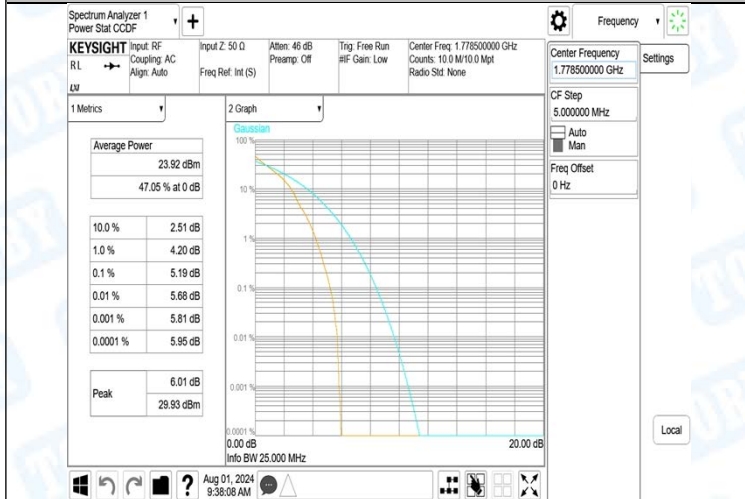
Band66-3MHz-16QAM-131987-1RB#0-PASS
