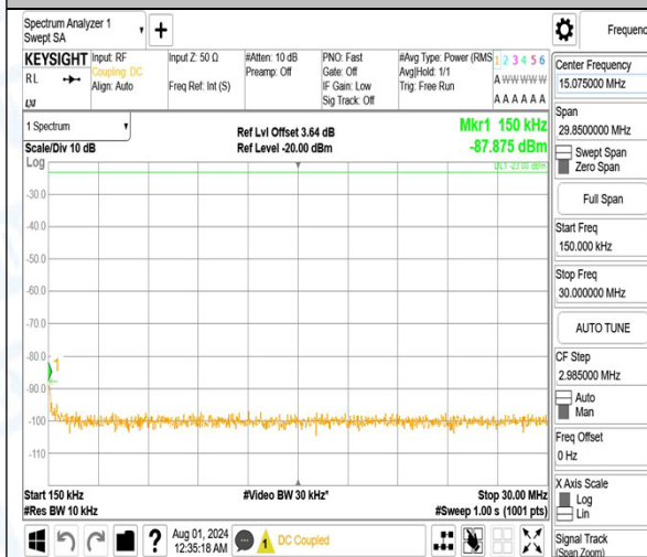
Band5_1.4MHz_QPSK_20525_6RB#0_1000~3000_1000~3000
