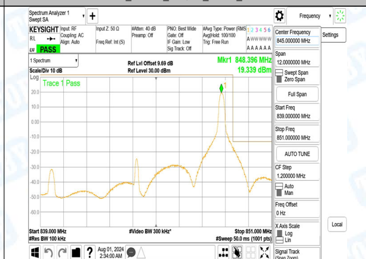
Band5 10MHz 16QAM 20600 1RB#49
