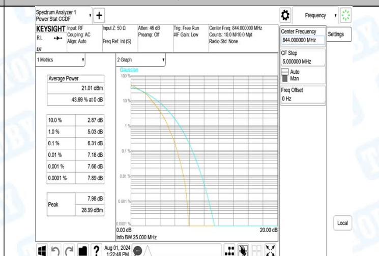
Band5-10MHz-16QAM-20600-27RB#0-PASS
