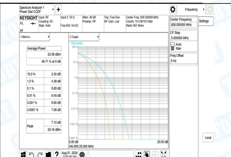
Band5-5MHz-QPSK-20525-25RB#0-PASS
