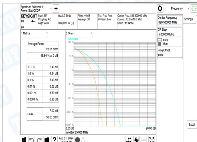
Band5-5MHz-QPSK-20525-1RB#0-PASS
