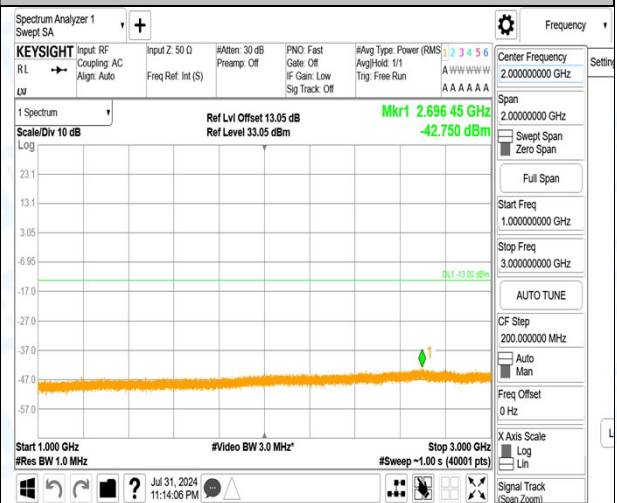
Band4_15MHz_16QAM_20025_1RB#0_1000~3000_1000~3000
