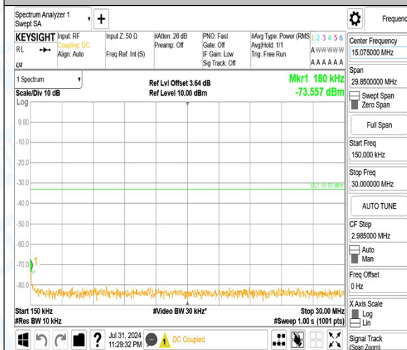
Band4_15MHz_QPSK_20325_75RB#0_0.15~30_0.15~30
