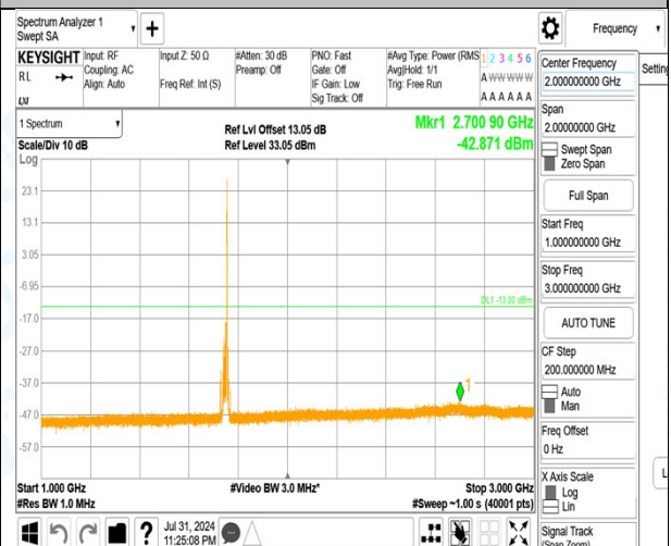
Band4_15MHz_QPSK_20325_1RB#74_1000~3000_1000~3000
