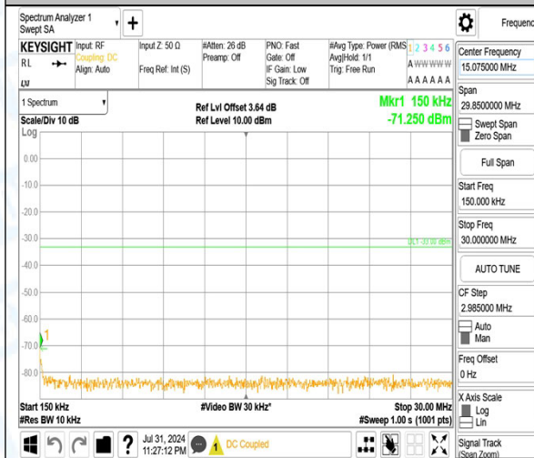
Band4_15MHz_QPSK_20025_75RB#0_0.15~30_0.15~30
