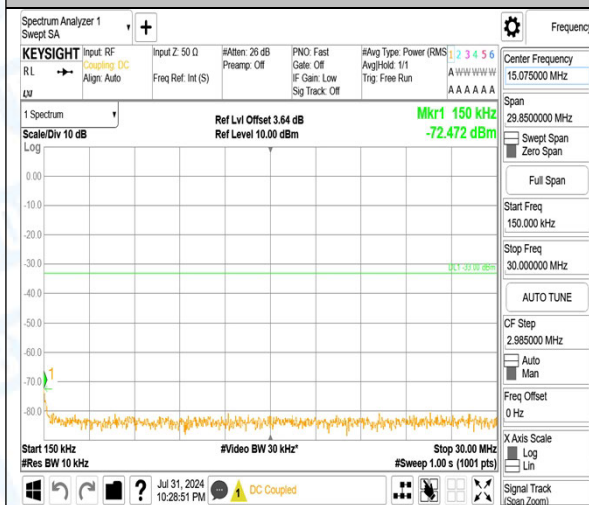
Band4_10MHz_16QAM_20175_1RB#0_0.15~30_0.15~30
