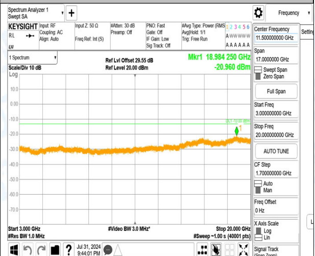
Band4_10MHz_QPSK_20000_1RB#0_0.15~30_0.15~30
