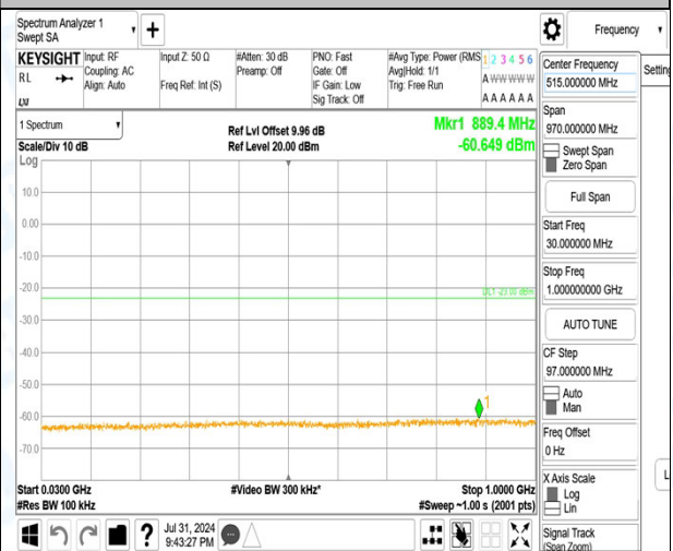
Band4_5MHz_16QAM_20375_25RB#0_3000~20000_3000~20000 0
