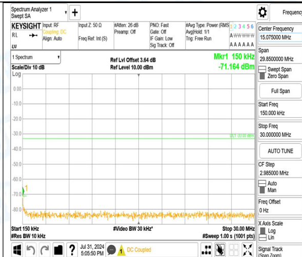
Band2_3MHz_16QAM_18900_1RB#14_1000~3000_1000~3000
