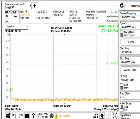
Band2_3MHz_QPSK_19185_1RB#14_1000~3000_1000~3000
